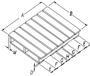
TYPE 4 WING PALLET
