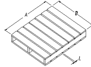
TYPE 3 REVERSIBLE PALLET
