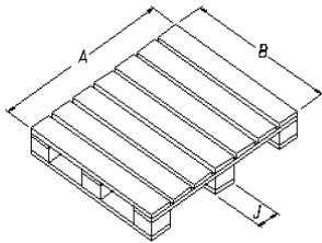
TYPE 7 BLOCK TYPE PALLET
