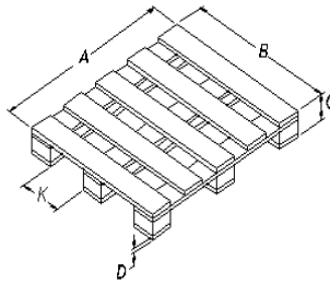
TYPE 8 BLOCK TYPE PALLET
