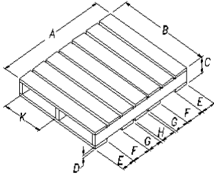
TYPE 1 TWO-WAY PALLET
