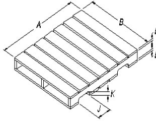
TYPE 2 FOUR-WAY PALLET
